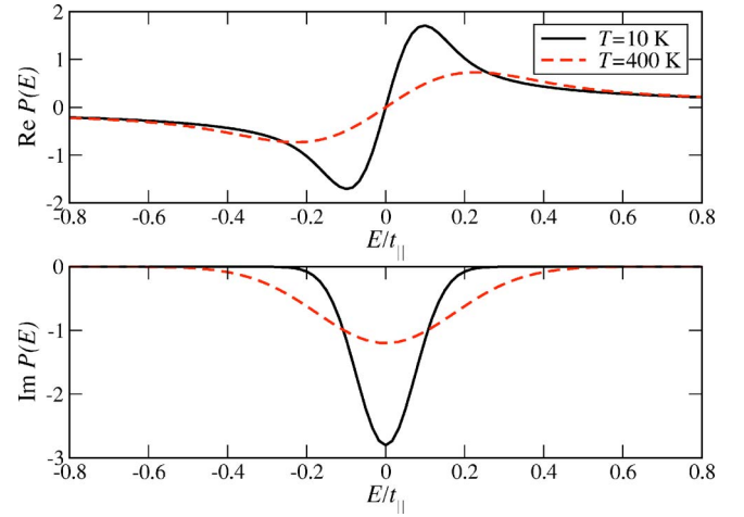
FIG. 4. (Color online) Temperature dependence of the real and imaginary parts of P(E) for N=20 , J_0/\omega_c=10 , t_\perp/t_\parallel=0.4 , \Gamma_{L/R}/t_\parallel=0.5 . With increasing temperature the slope of the real part near E=0 decreases and the imaginary part broadens and loses intensity. A similar qualitative dependence on J_0 was found (not shown).
