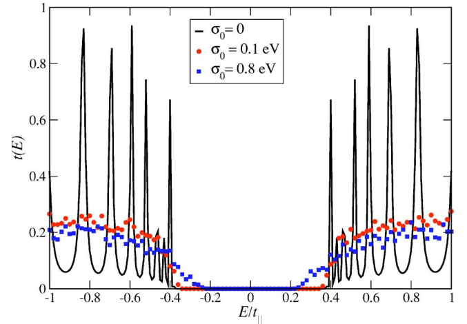
FIG. 8. (Color online) Transmission function in presence of thermal disorder in the central chain. Parameters: N=20 , J_0/\omega_c=5 , t_{\perp}/t_{\parallel}=0.5 , \Gamma_{L/R}/t_{\parallel}=0.15 , T=10 \text{ K} . The transmission on the side bands decreases when the disorder becomes stronger, but the pseudogap is still seen, although it is partially reduced with increasing disorder.
