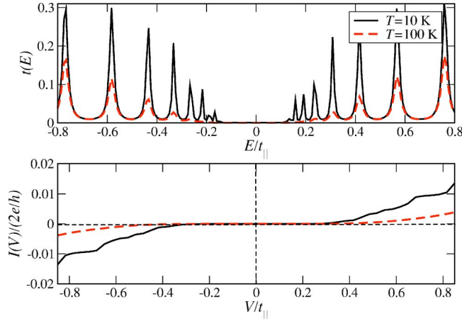
FIG. 3. (Color online) Electronic transmission and corresponding current in the weak-coupling limit with Ohmic dissipation ( s = 1 ) in the bath. Parameters: N=20 , J_0/\omega_c=0.2 , t_\perp/t_\parallel=0.6 , \Gamma_{L/R}/t_\parallel=0.5 .
