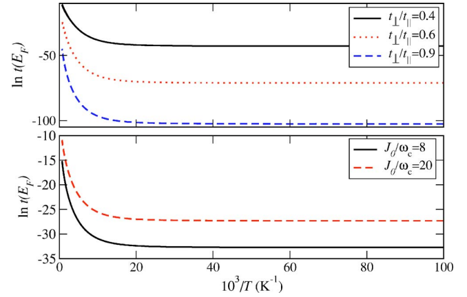
FIG. 6. (Color online) Arrhenius plot of t(E=E_F) for different transversal couplings t_\perp (upper panel) and electron-bath couplings J_0/\omega_c (lower panel). Parameters: N=20 , t_\perp/t_\parallel=0.5 , \Gamma_{L/R}/t_\parallel=0.25 .
