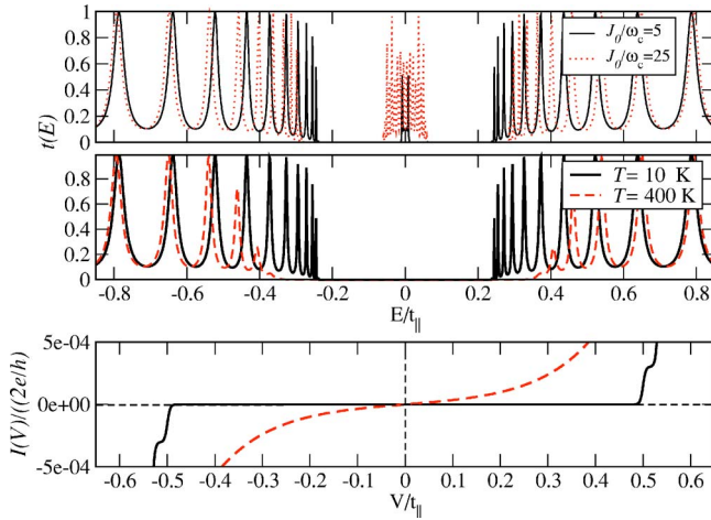
FIG. 5. (Color online) Upper panel: t(E) with \text{Im} P(E)=0 ; the intensity of the resonances on the central narrow band is strongly dependent on J_0/\omega_c and k_B T (not shown). Temperature dependence of t(E) with full inclusion of P(E) (middle panel) and corresponding current (lower panel) for N=20 , J_0/\omega_c=5 , t_\perp/t_\parallel=0.5 , \Gamma_{L/R}/t_\parallel=0.2 . The pseudogap increases with temperature.
