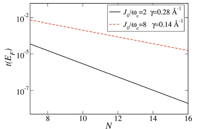
FIG. 7. (Color online) Chain length dependence of the transmission function at the Fermi energy for different electron-bath interaction strengths. Parameters: t_\perp/t_\parallel=0.125 , \Gamma_{L/R}/t_\parallel=0.15 , T=200 K.
